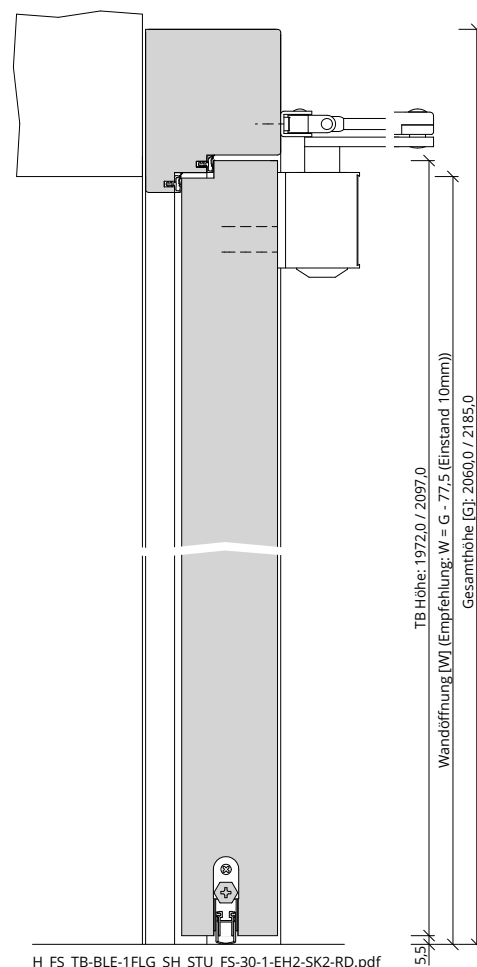
H_FS_TB-BLE-1FLG_SH_STU_FS-30-1-EH2-SK2-RD.pdf
