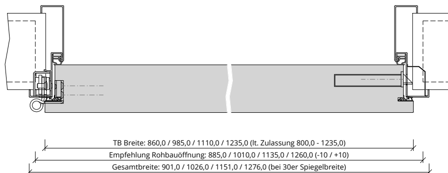
Q_FS_TB-ST-1FLG_SH_GEF_T30RS-1-SK4-13_AC.dwg
