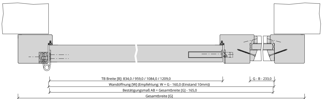
Q_FS_TB-BLE-1FLG_WF3-V1_STU_FS-30-1-RD.pdf
