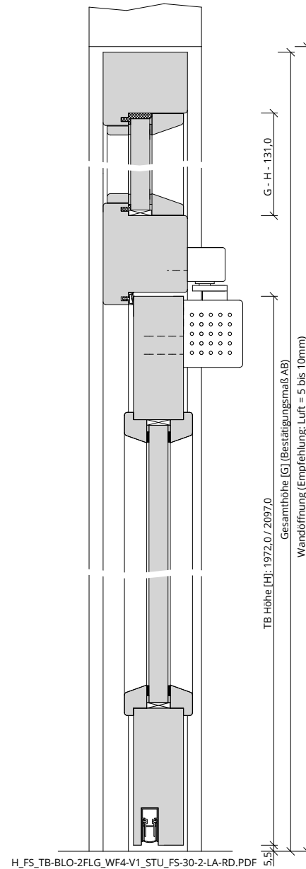
H_FS_TB-BLO-2FLG_WF4-V1_STU_FS-30-2-LA-RD.PDF
