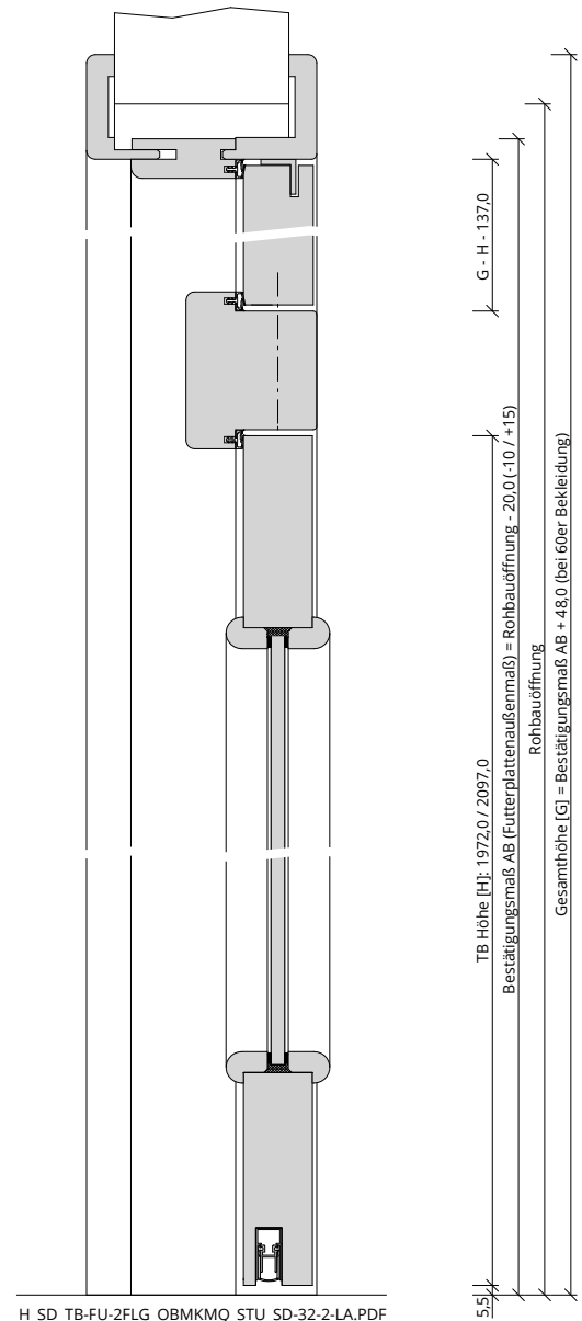
H_SD_TB-FU-2FLG_OBMKMQ_STU_SD-32-2-LA.PDF
