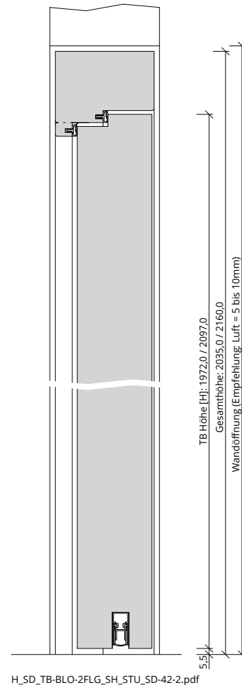
H_SD_TB-BLO-2FLG_SH_STU_SD-42-2.pdf
