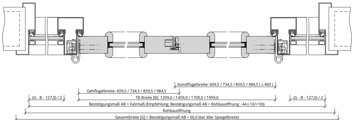
Q_SD_TB-ST-2FLG_WF2_STU_SD-32-2-LA.pdf
